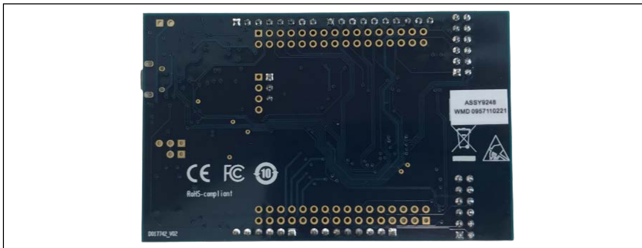
Figure 4. Identification of the Serial Number on the FPB-RA2E1 Board
