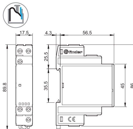
Type 70.92 Screw terminal
