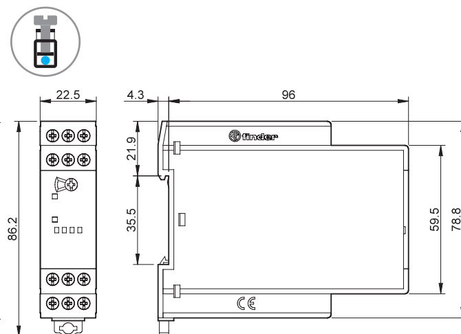
Type 70.92 Screw terminal
