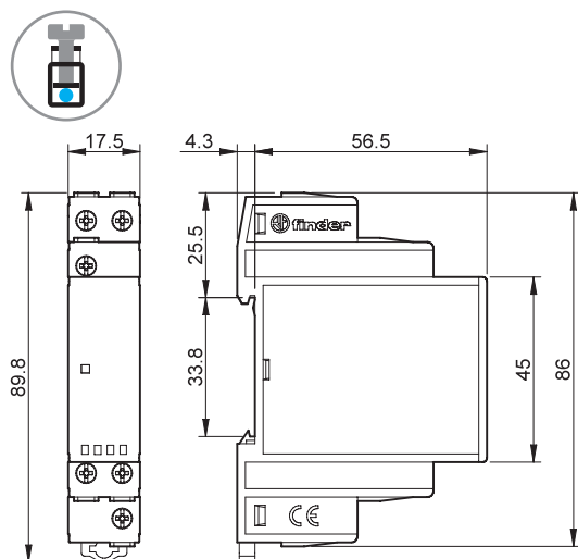
Type 70.62 Screw terminal
