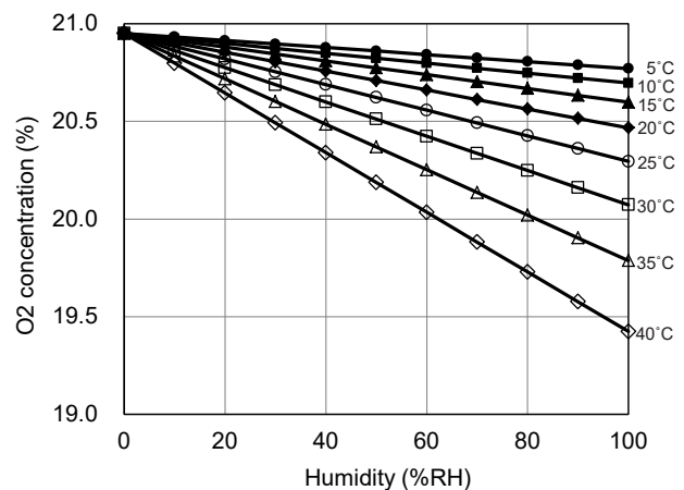
Fig. 6 - Effect of humidity on O2 concentration
