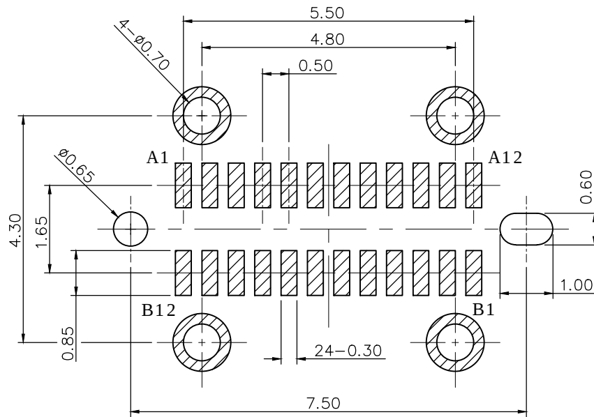
RECOMMENDED LAYOUT ( TOP VIEW ) GENERAL TOLERANCE: \pm 0.05\text{mm}
