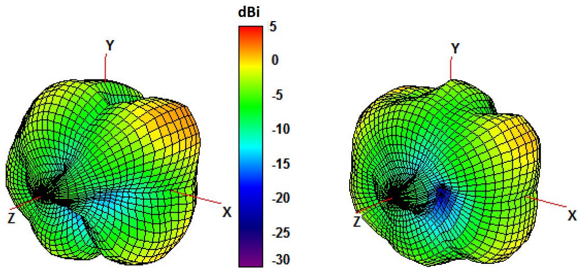
1950 and 2100 MHz Radiation pattern
