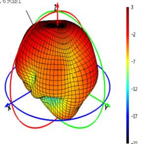
Phi=0 Freq=2600MHz
