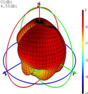
Phi=0 Freq=2140MHz
