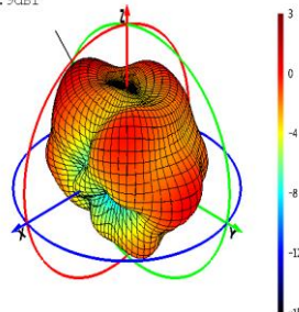
Phi=0 Freq=2450MHz
