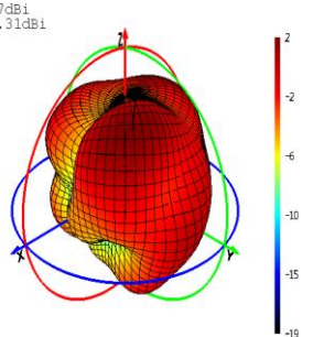
Phi=0 Freq=2350MHz
