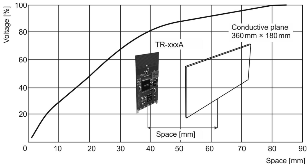
Figure 5: Parallel arrangement
