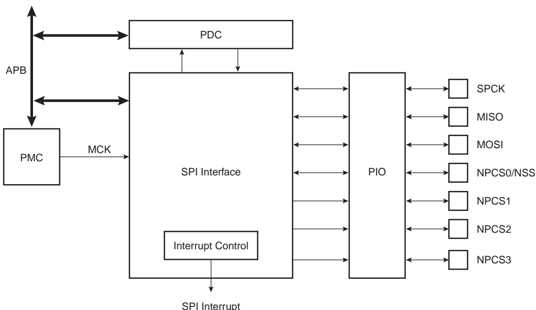
Figure 32-1. Block Diagram
