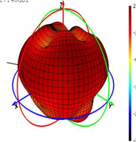
Phi=0 Freq=1740MHz
