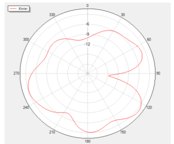
Theta=90 Freq=830MHz
