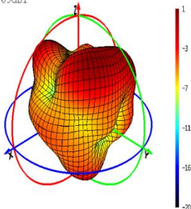
Phi=0 Freq=900MHz
