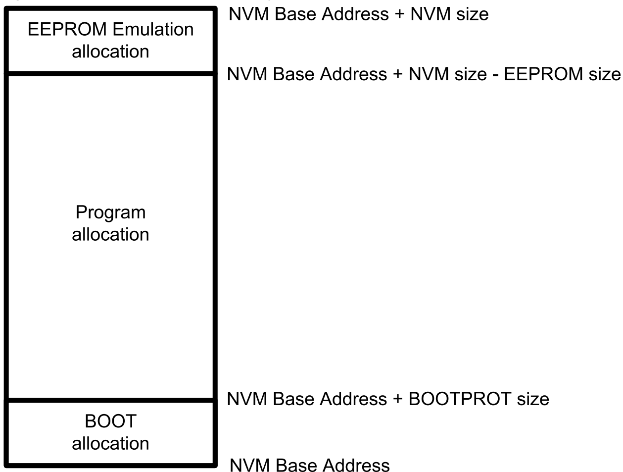
Figure 27-4. EEPROM Emulation and Boot Loader Memory Allocation
