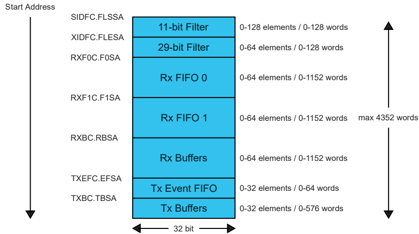
Figure 34-12. Message RAM Configuration
