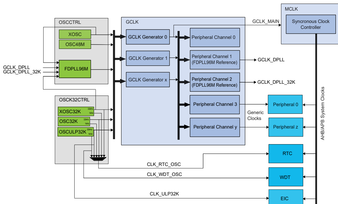
Figure 15-1. Clock distribution
