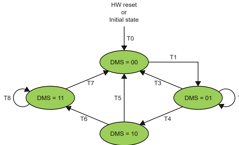
Figure 34-9. Debug Message Handling State Machine
