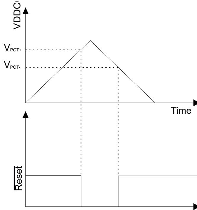
Figure 49-1. POR Operating Principle
