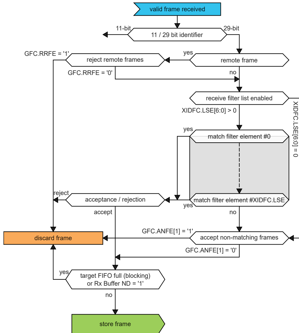
Figure 34-6. Extended Message ID Filtering
