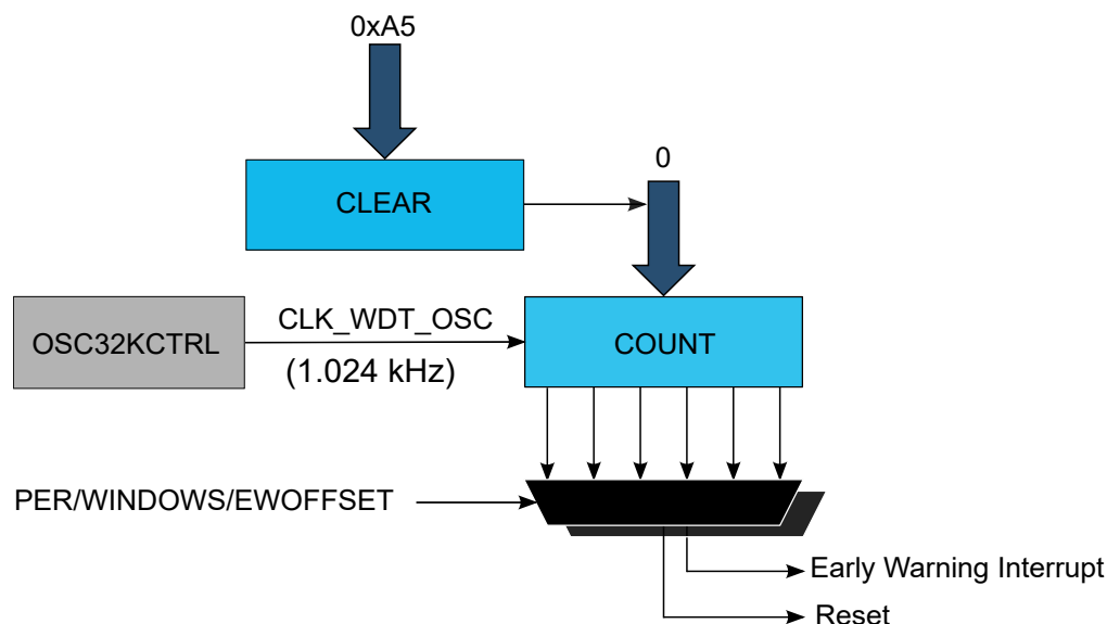
Figure 23-1. WDT Block Diagram
