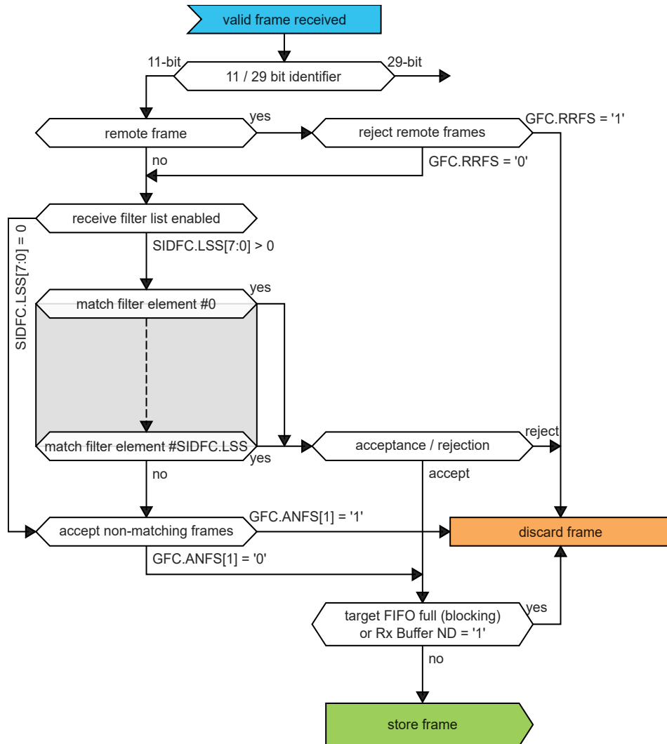
Figure 34-5. Standard Message ID Filtering
