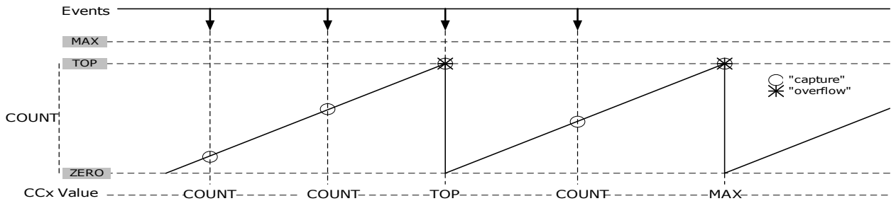
Figure 35-15. Time Stamp
