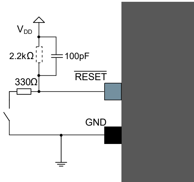
Figure 53-5. External Reset Circuit Schematic
