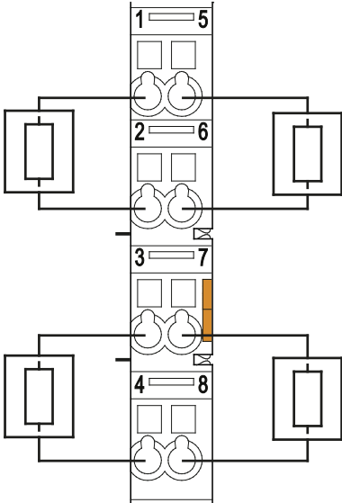
Figure 11: Connecting Diagram
