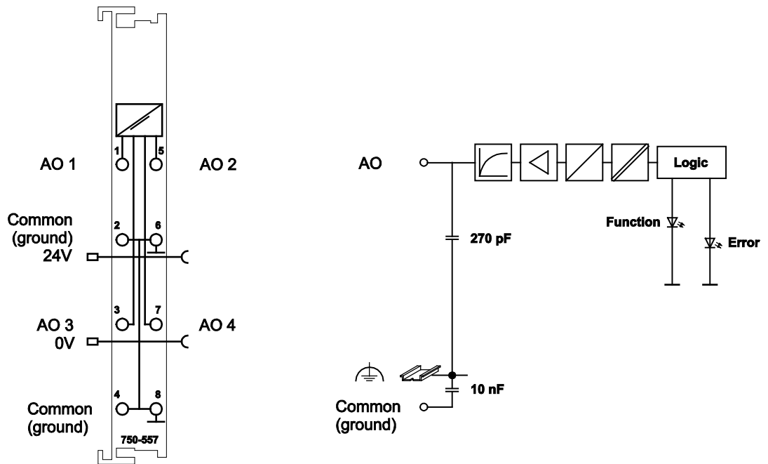
Figure 6: Schematic Diagram
